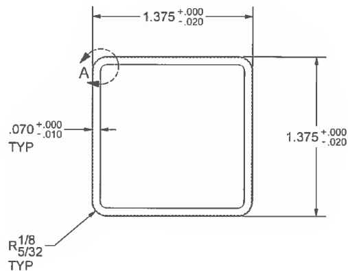
1.375" x 1.375" Picket
