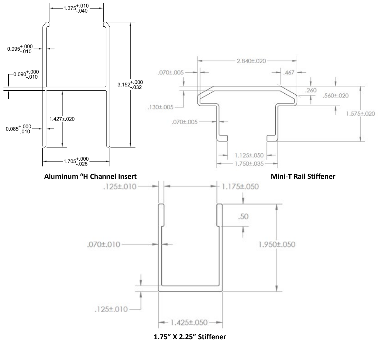
FIGURE 2 – ALUMINUM INSERTS
