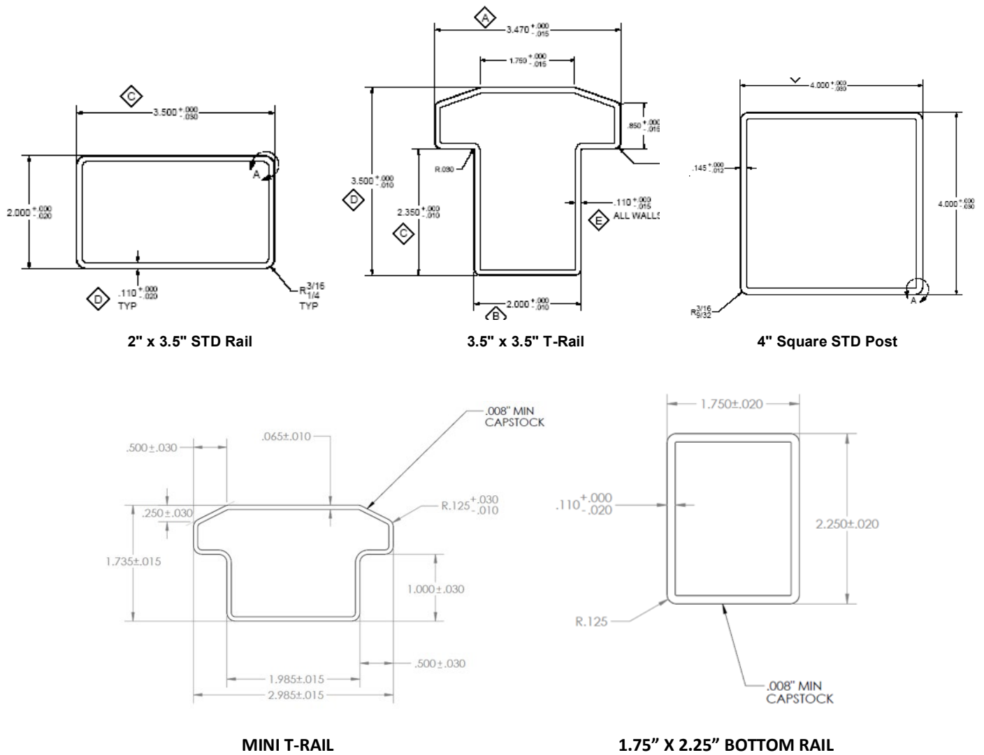
FIGURE 1 – PVC PROFILE DRAWINGS
