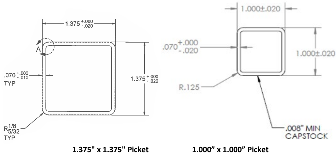
FIGURE 3 – PVC PICKET PROFILES
