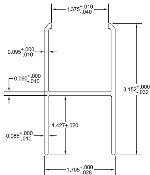
FIGURE 1 – PVC PROFILE DRAWINGS
