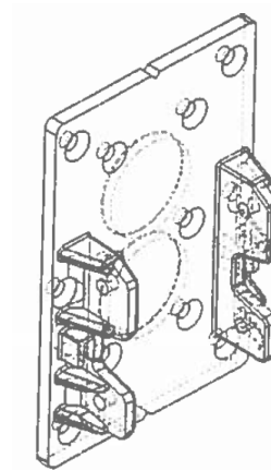
Eclipse 3-1/2 x 3-1/2" T-Rail Straight Top Bracket (Also used for T-Rail Stair Top)
