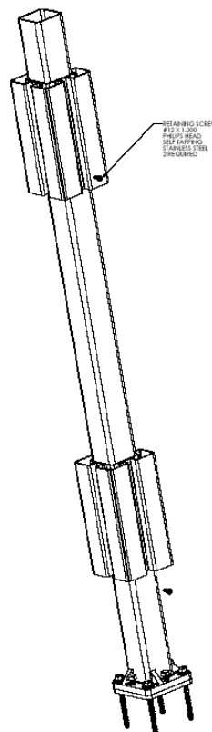
FIGURE 12– STEEL POST MOUNT TOWER
