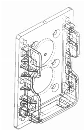
Eclipse 2" x 3-1/2" STD Top and Bottom Rail Straight Bracket (Also used for T-Rail Level Bottom Rail)
