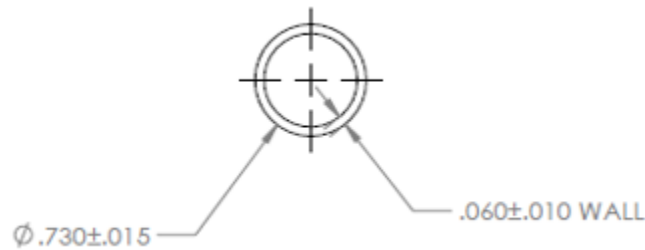
3/4" ALUMINUM PICKET
