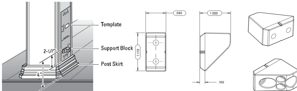
FIGURE 12 - RADIANCERAIL® SUPPORT BLOCK
