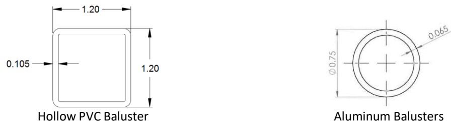
FIGURE 10 - RADIANCE RAIL® EXPRESS BALUSTER PROFILE
