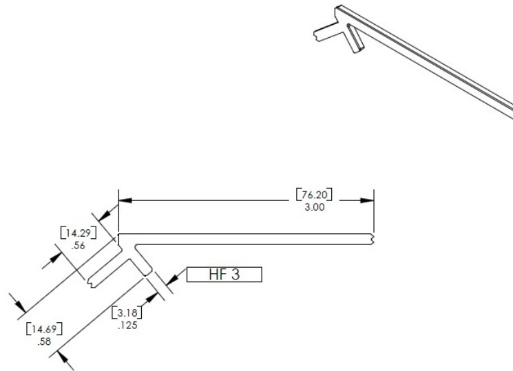
FIGURE 6 – HIDFAST FASTENER
