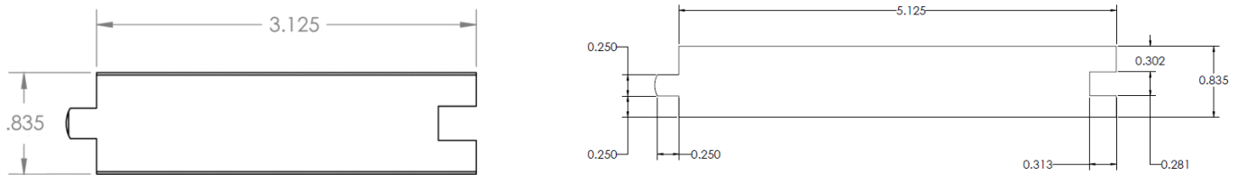
FIGURE 4 – DECKORATORS® PORCH PROFILES (TONGUE AND GROOVE)
