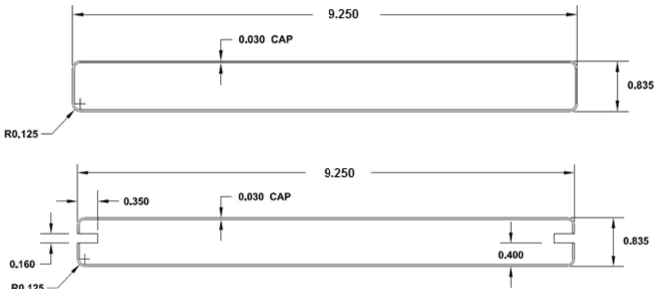
FIGURE 7 – 9.25" DECKORATORS® VOYAGE VARIED-PLANK DECKING
