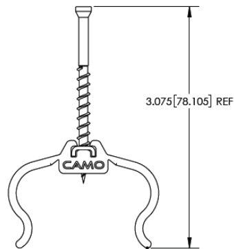
EdgeClip Hidden Fastener System
