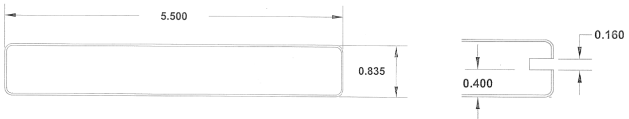
FIGURE 3 – DECKORATORS® (VAULT, VOYAGE, SUMMIT, EXCURSION, AND FRONTIER) AND EOVATIONS™ TRACTIO DECK BOARD PROFILES
