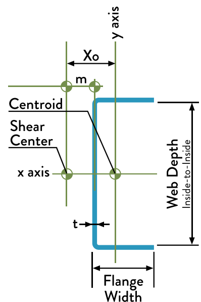
Track Cross Section
