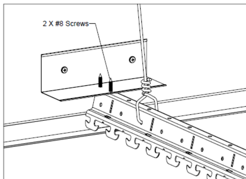
CARRIER CHANNEL
