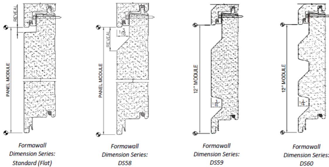
Figure 1 – Formawall Series/Profiles
