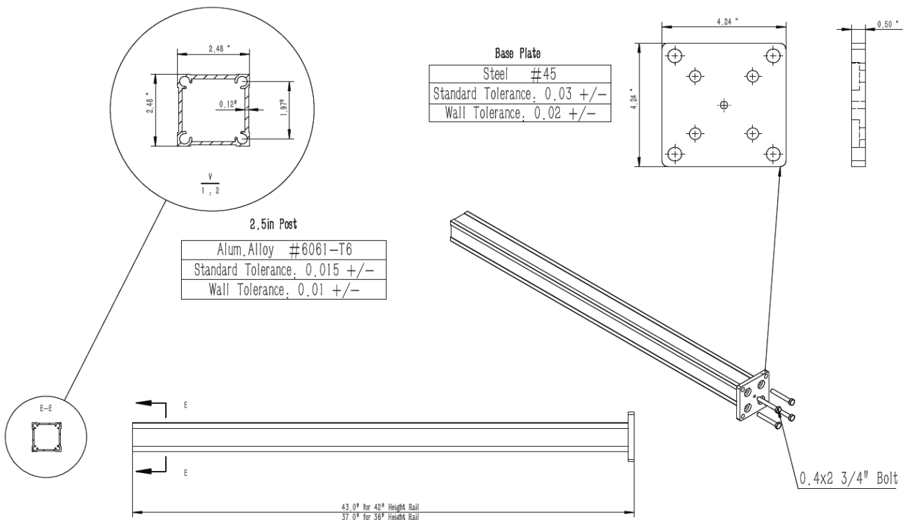
FIGURE 4 - 2.5 INCH POST
