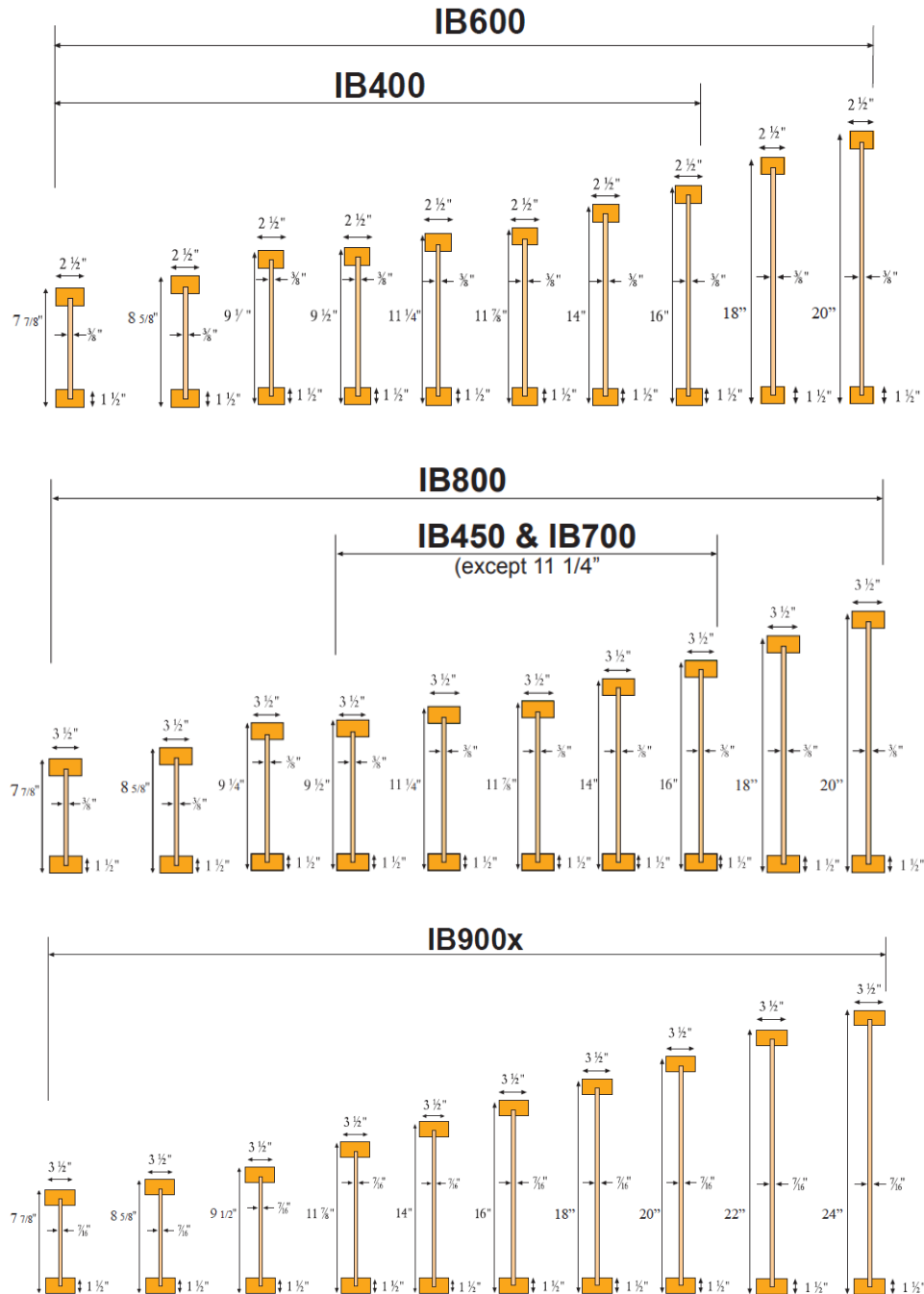
FIGURE 1 – I-JOIST ILLUSTRATIONS
