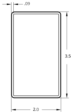
Top Rail
