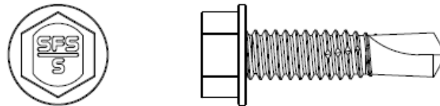
FIGURE 2 – 1/4-20 SD4 BI-MET 300® SCREW
