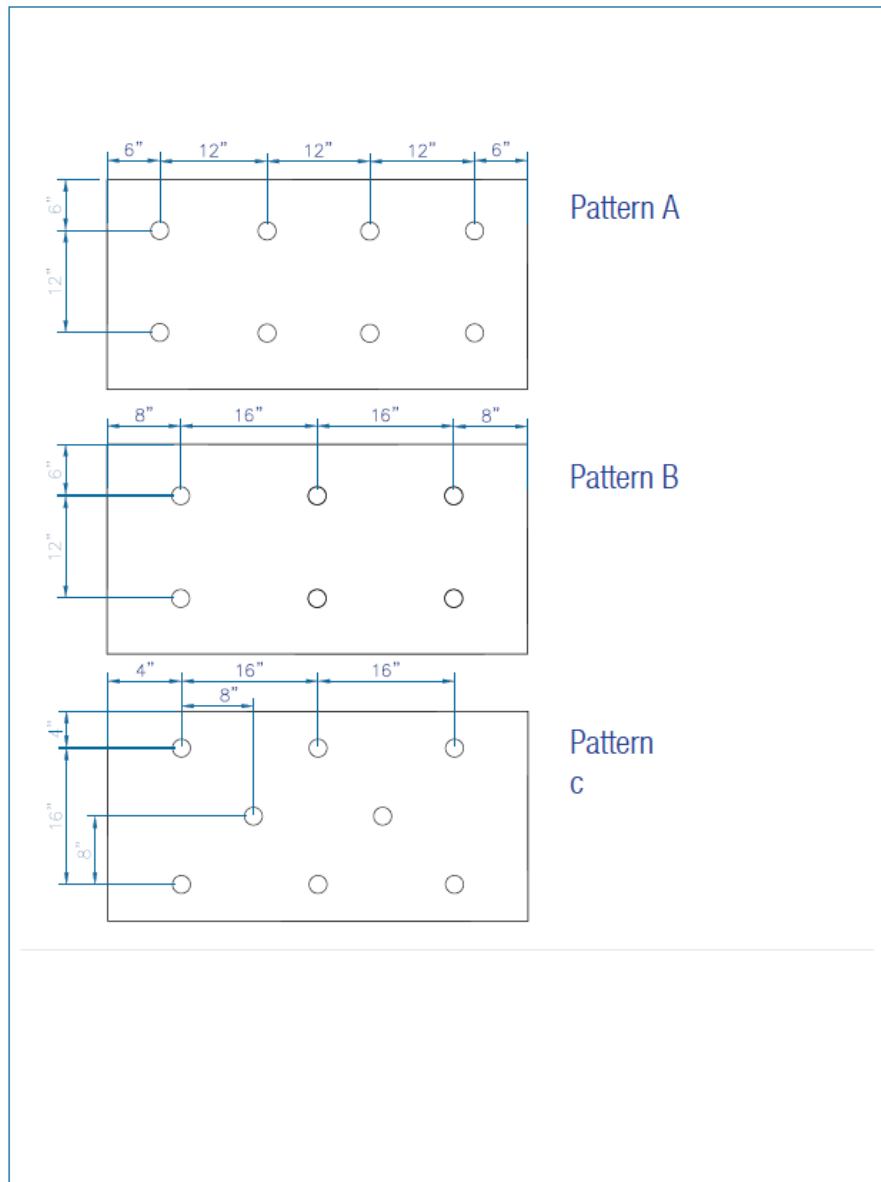
Figure 1 – Fastening Patterns for Insulation Board See Table 3
