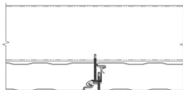
ONE V6 X-SPAN CLIP AT EACH SUPPORT WITH ONE FACE-TO-CLIP FASTENER AT PANEL ENDS ONLY
