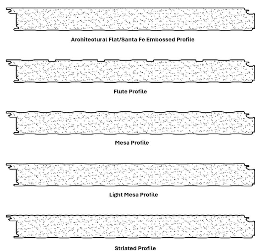
Figure 1 – CF Wall Panel with PIR Core Profiles
