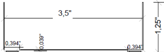
Figure 13: UMS EQ Track 350T125-15 (25 EQ)
