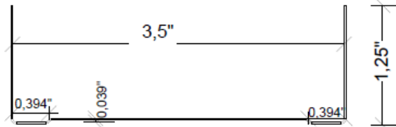
Figure 18: UMS EQ Track 350T125-15 (20 EQ)
