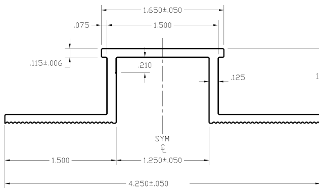
Figure 3 – Hat Channel
