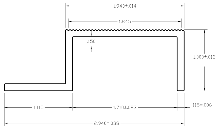
Figure 4 – J-channel
