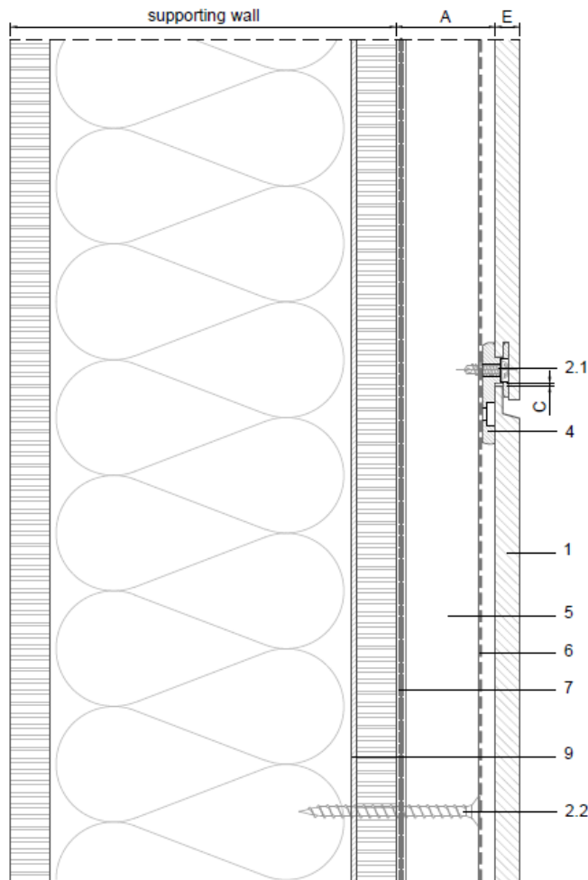
Figure 9 – Typical Installation – Horizontal Joint - Siding System
