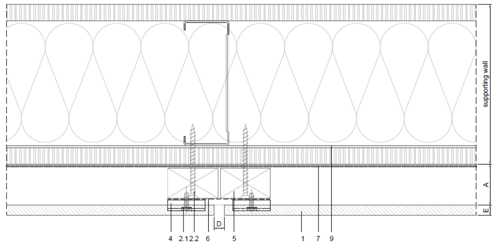
Figure 10 – Vertical Joint – Siding System
